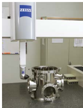
CNC CMM (coordinate measurement machine) inspection
