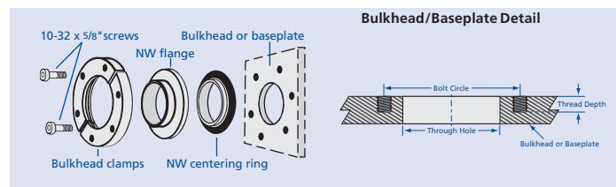
Bulkhead/Baseplate Detail
