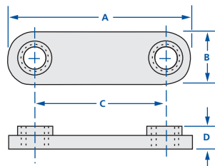
Plate Nut for Flanges larger than 2 \frac{3}{4} (69.85)
