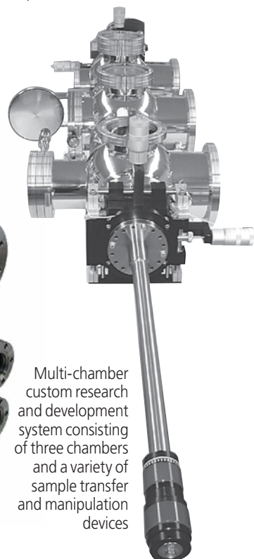
Cornell University Physics Department surface science chamber
