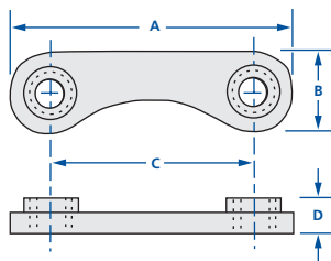
Plate Nut for 1 \frac{1}{3} (33.78) and 2 \frac{3}{4} (69.85) Flanges
