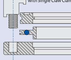
B. Optional Fastener/ Tapped Nonrotatable with Single Claw Clamp
