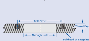
Bulkhead/Baseplate Detail
