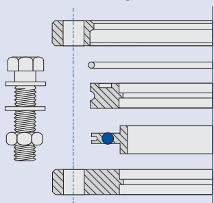
C. Optional Fastener/ Nonrotatable with Rotatable Bolt Ring and Bolts
