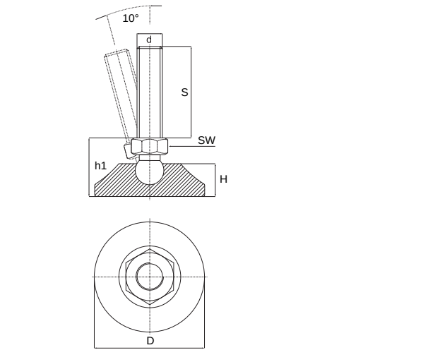
PlacoGrip® Machine levelling feet, adjustable, of steel, foot painted
