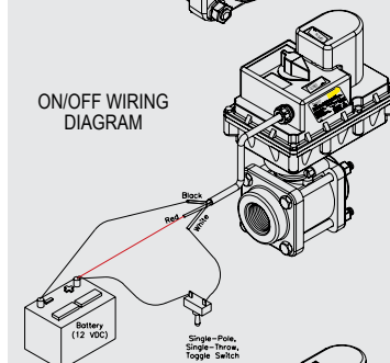
REGULATING WIRING DIAGRAM
