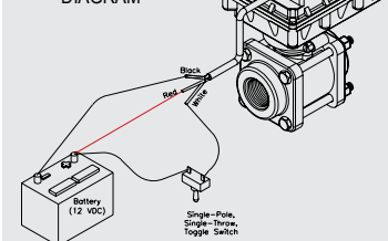
ON/OFF WIRING DIAGRAM
