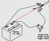
REGULATING WIRING DIAGRAM
