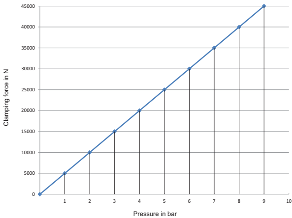
Diagramme clamping force BSPD-420
