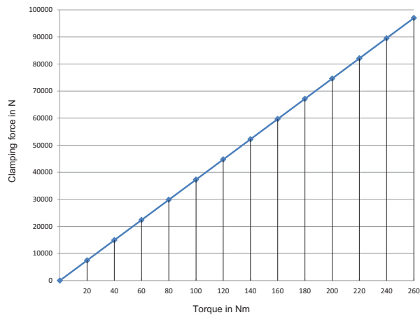
Clamping force - torque BSMG-400
