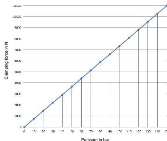
Diagramme clamping force BSH-290
