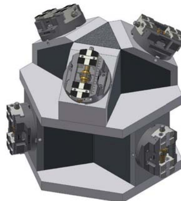
5-axis pyramid tombstone with 6 clamping positions
