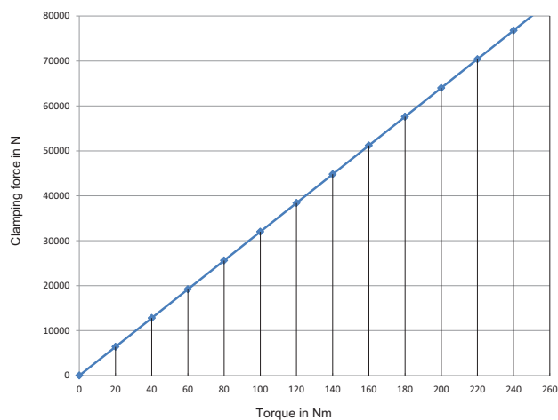
Clamping force - torque BSM-400
