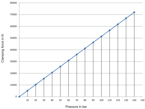
Diagramme clamping force BSH-500
