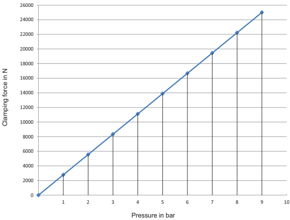
Diagramme clamping force BSP-160
