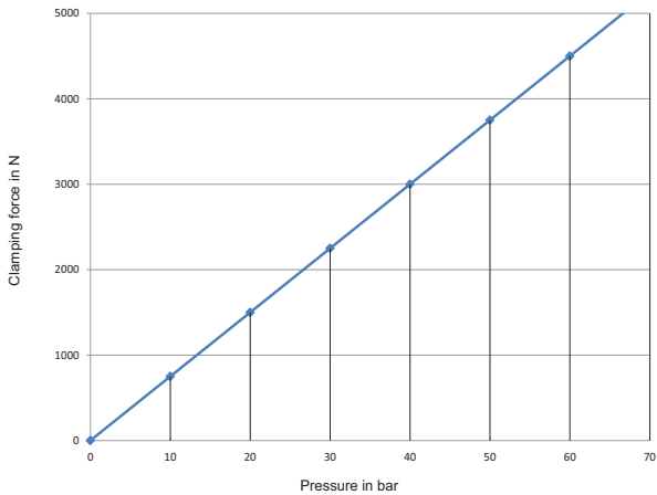
Diagramme clamping force BSH-64
