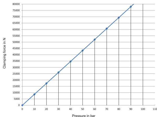
Diagramme clamping force BSH-250
