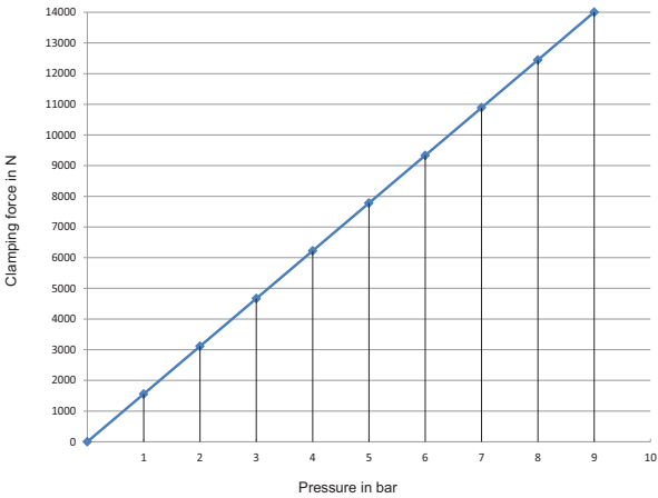
Diagramme clamping force BSP-100
