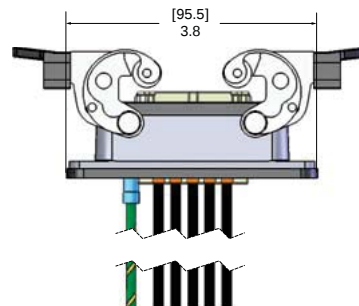
10 Pole Double Lever
