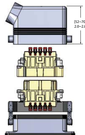
Side Entry Squich Inserts
