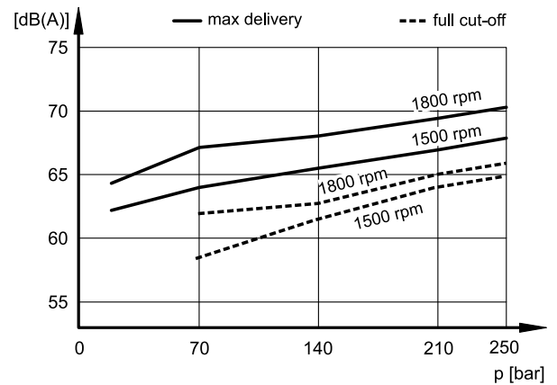
NOISE LEVEL
